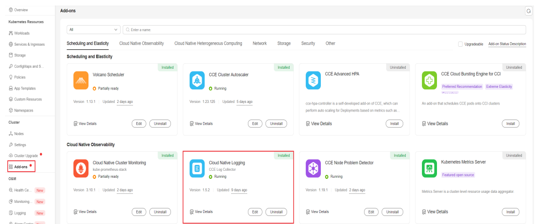
Figure 4-1 Viewing the installed add-on version
